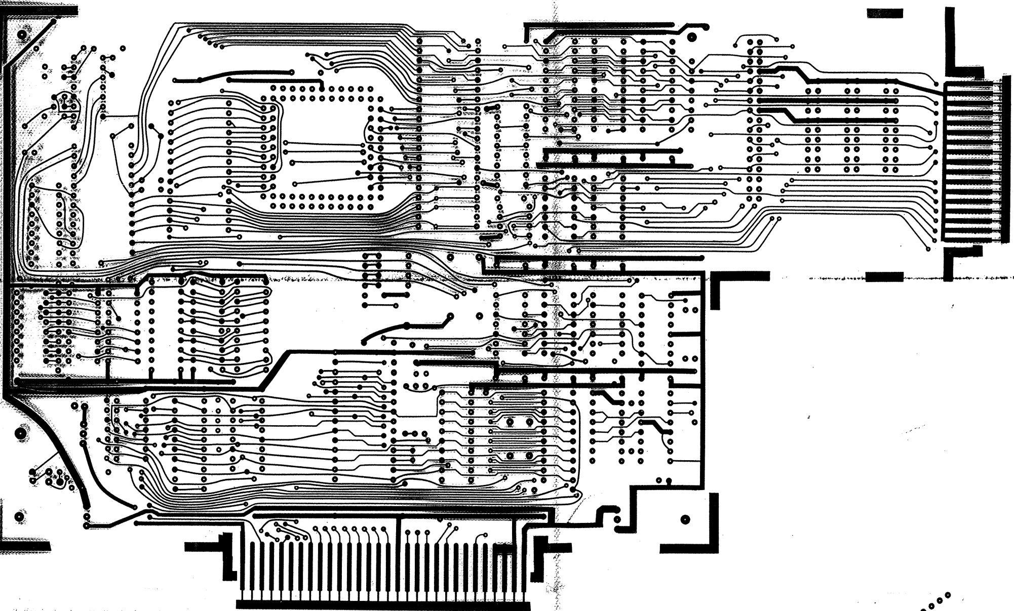
Myarc HFDC - circa 1987
